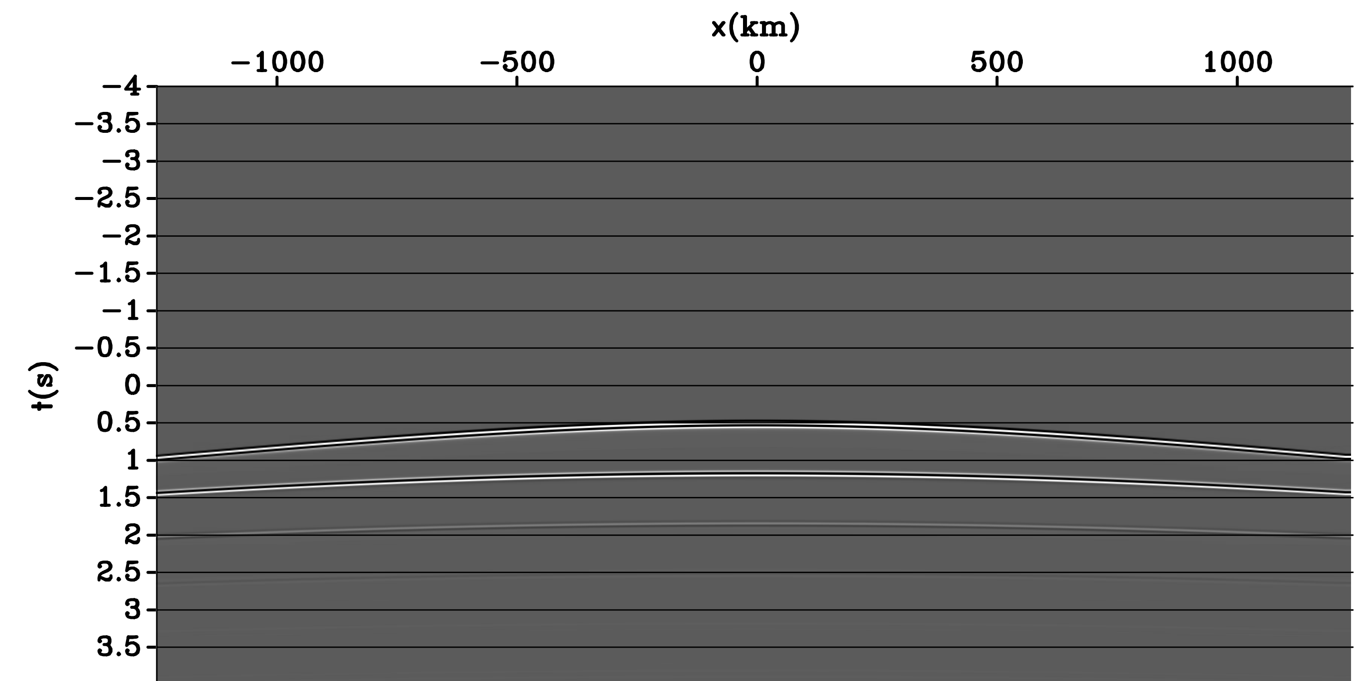
Modeled virtual source
