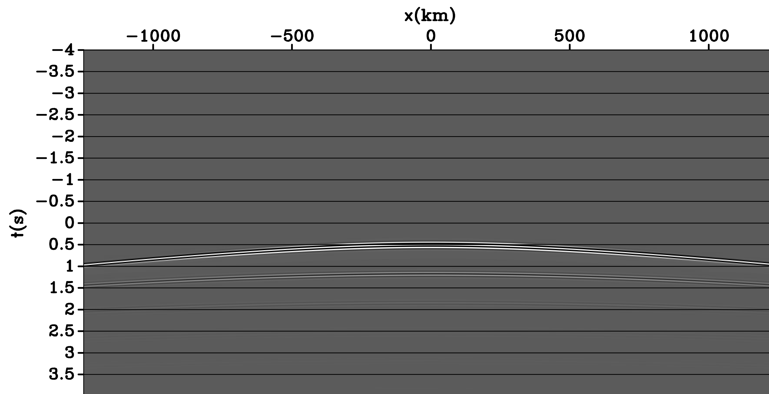
Reconstructed virtual source
