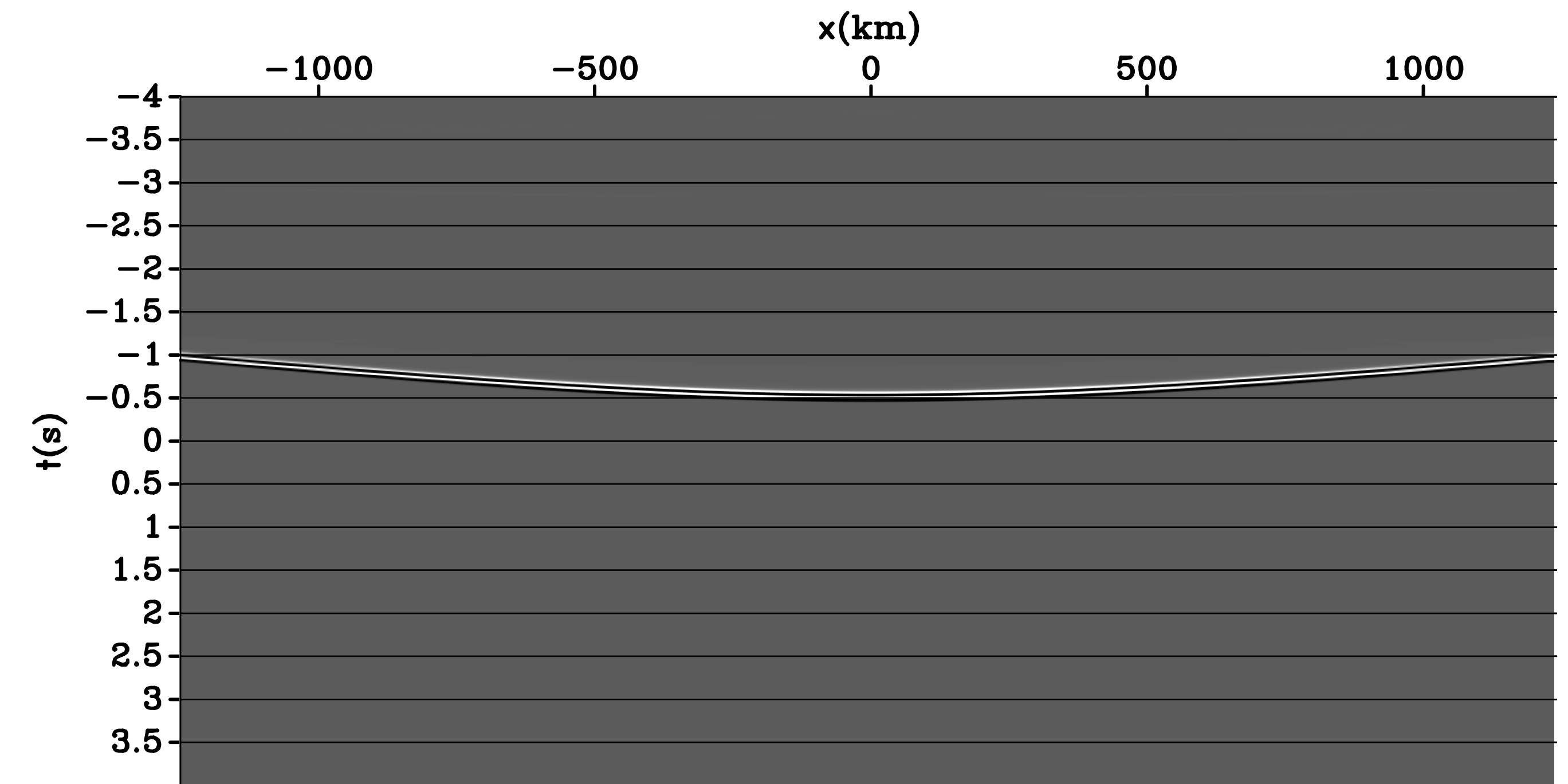
Direct arrival of virtual source
