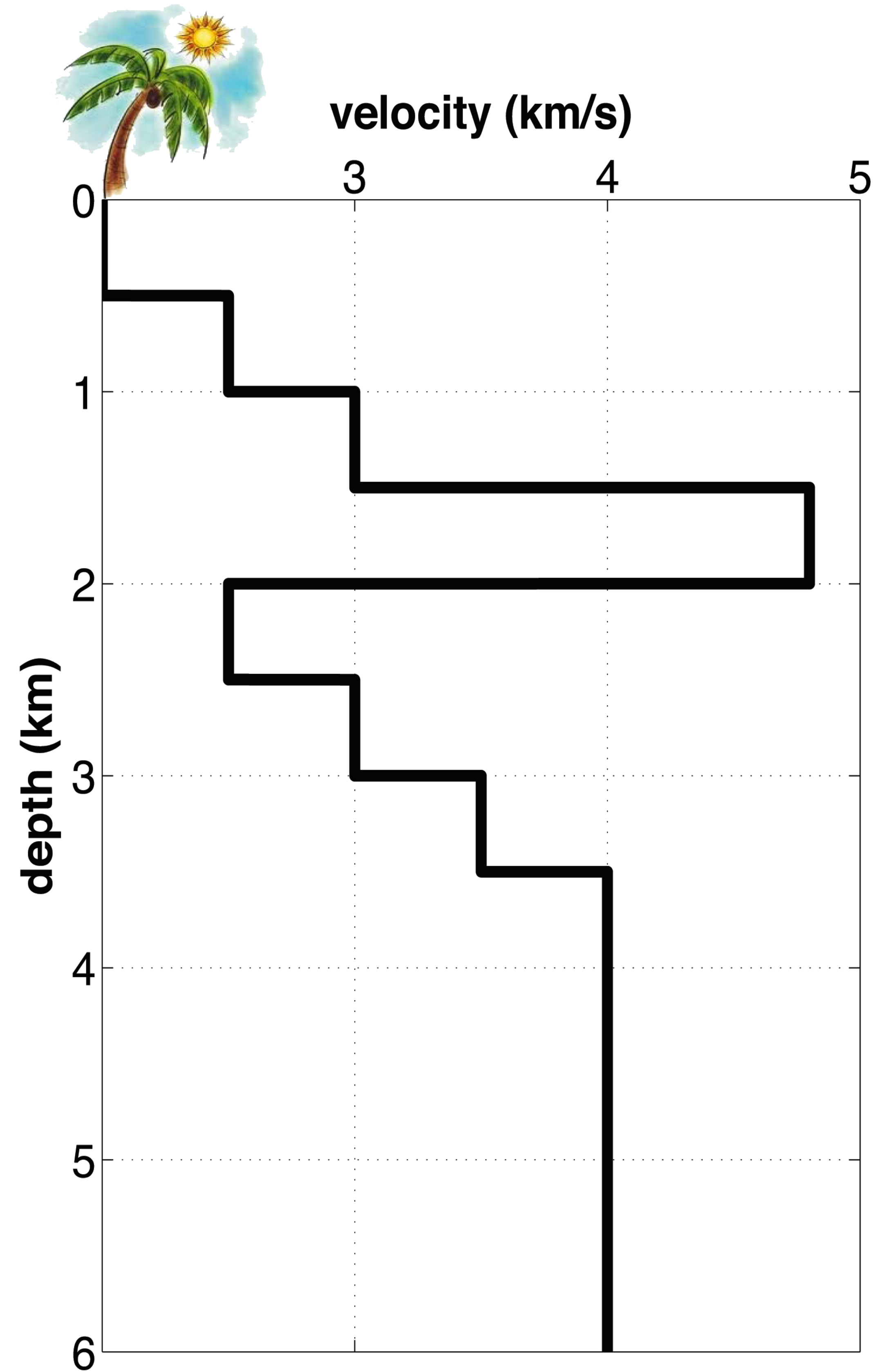
Velocity model
