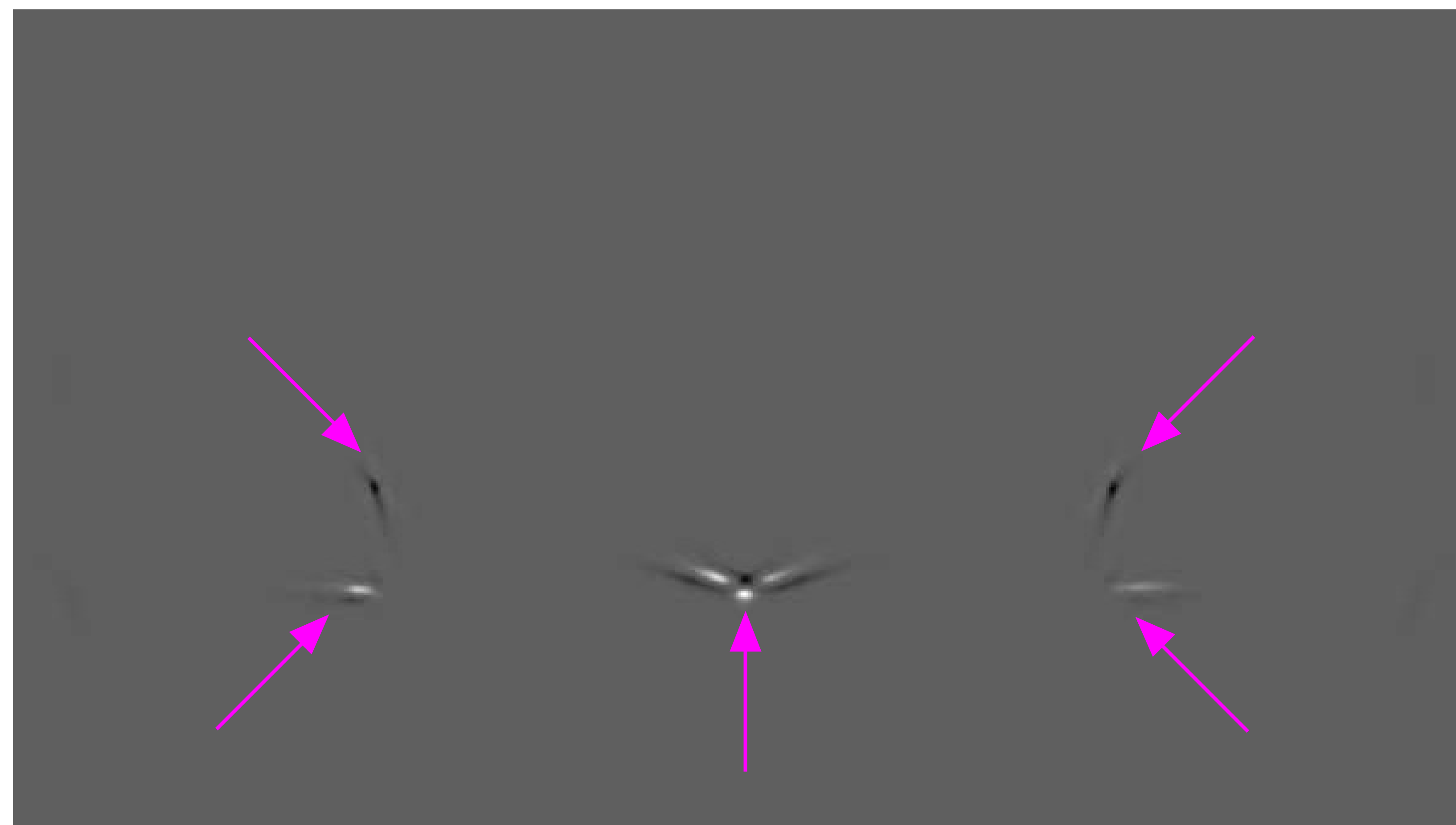
Diffraction image
