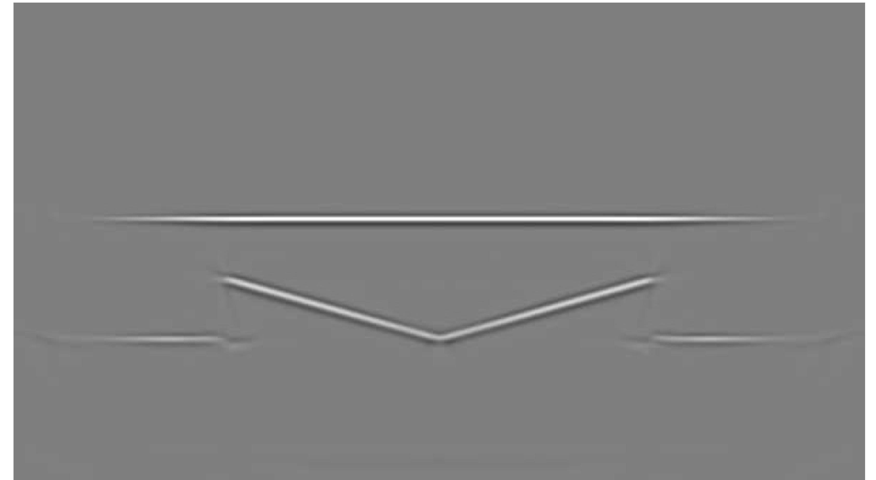
Conventional Kirchhoff migration
